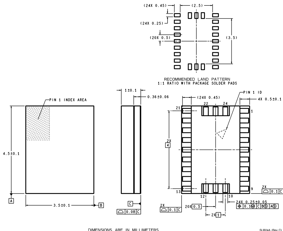
Molded CSP, JEDEC Plastic Package (SLB24A) Order Number LMX2350SLB or LMX2352SLB NS Package SLB24A
